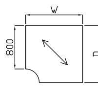
Corner Workstation
